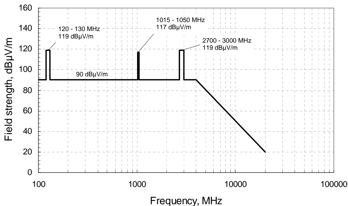
Figure 5-15 Field strength of launch vehicle and cosmodrome electromagnetic emissions in the adapter plane without payload fairing.
