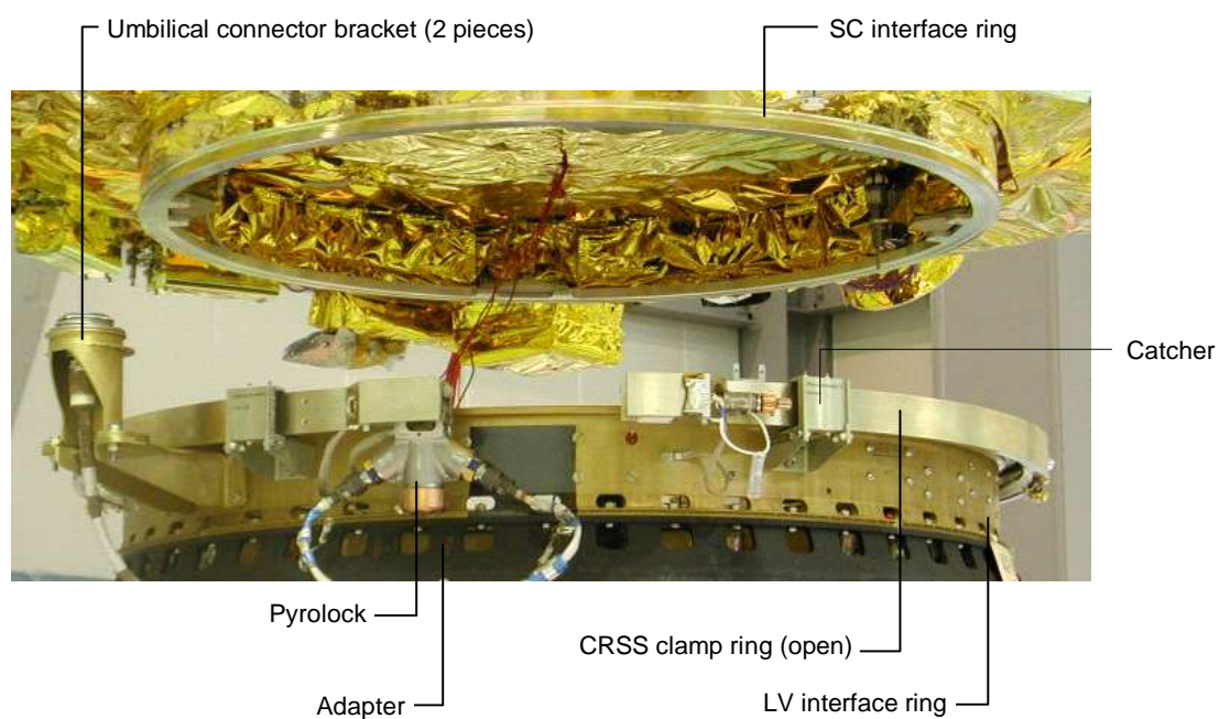
Figure 4-4 CASA CRSS Clamp Ring Separation System installation with KSRC pyrolock.
