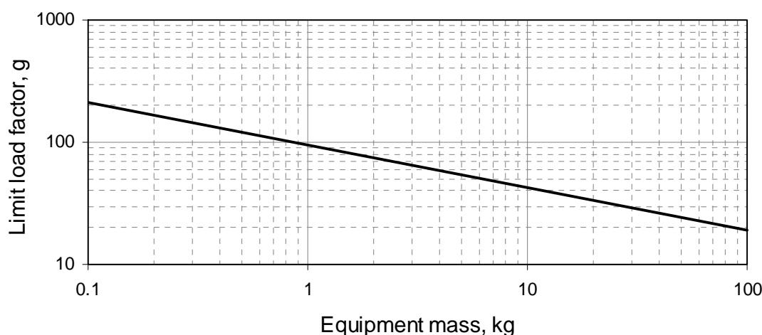
Figure 6-1 Typical limit load factors for initial dimensioning of secondary structures and equipment brackets.
