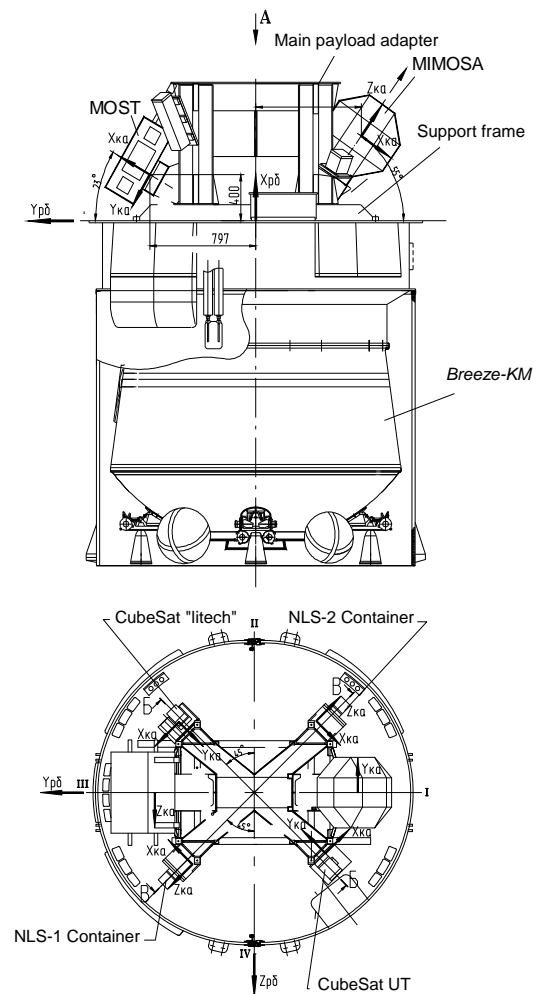
Figure 4-1 Multiple payload accommodation for MOM without main payload.
