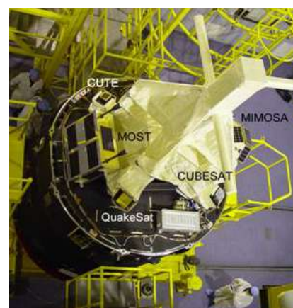
Figure 4-2 Integrated MOM payload with main payload simulator.
