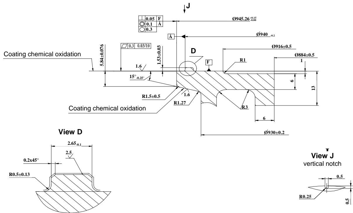
Figure 4-10 CASH 937 SRF clamp band cylindrical payload adapter. (a) Side view. (b) Launch vehicle interface ring detail.
