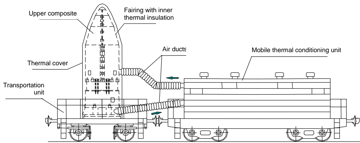
Figure 5-12 Thermal conditioning of the upper composite during transportation.
