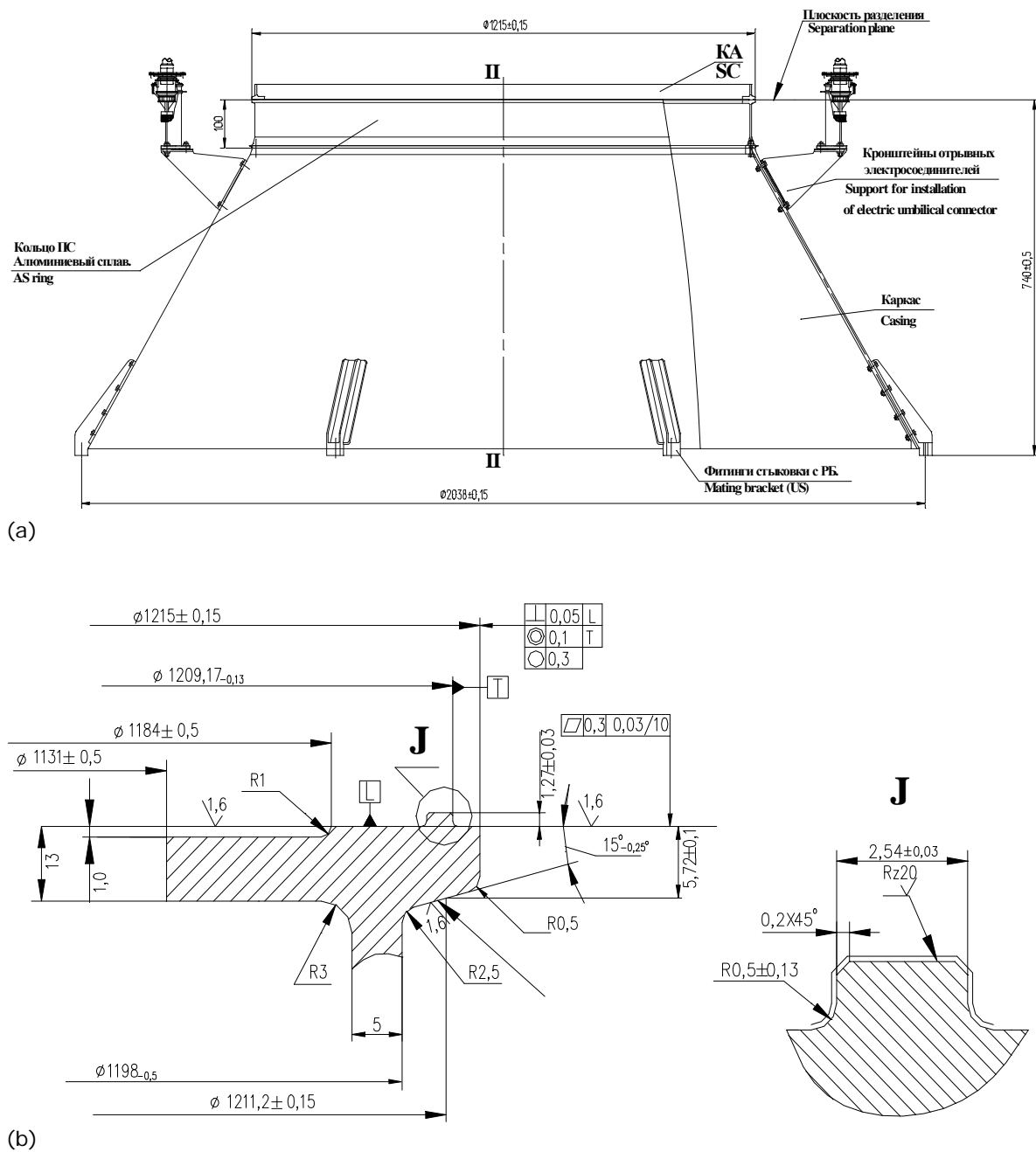
Figure 4-11 CASA CRSS 1194 SRF clamp band conical payload adapter system (Komsat-2). (a) Side view. (b) Launch vehicle interface ring, detail.
