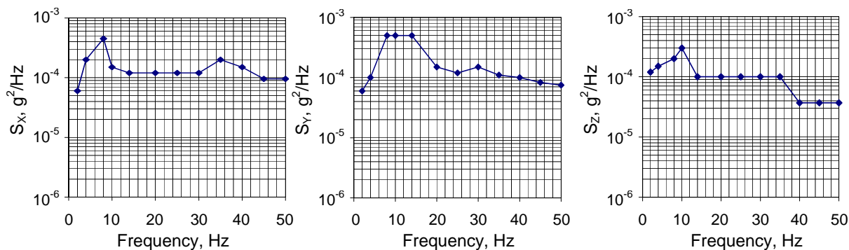
Figure 5-11 Random vibration power spectrum acting on the spacecraft during upper composite transportation.
