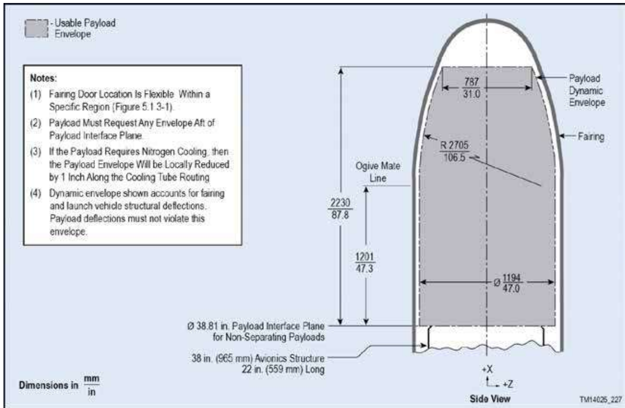
Figure 5.1.1.1-1. 50" Payload Fairing Dynamic Envelope with 38" (97 cm) Diameter Payload Interface
