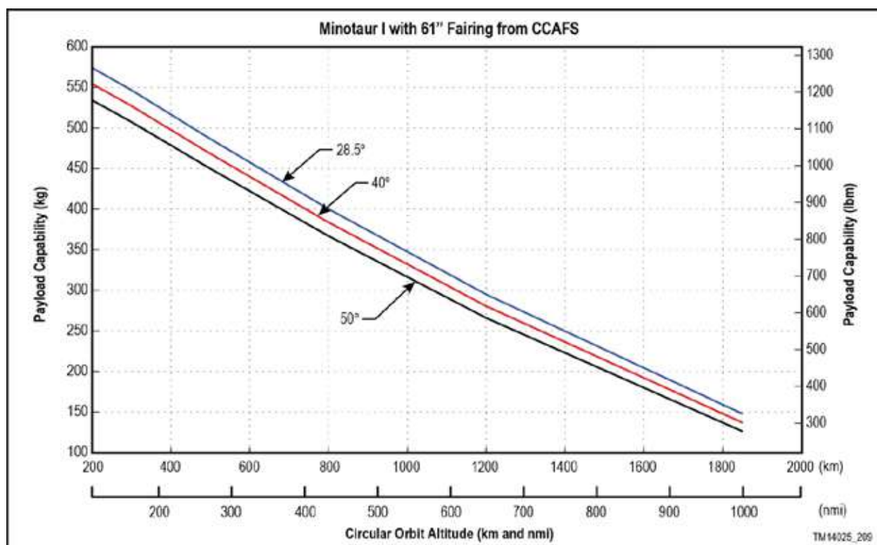
Figure 3.3-7. Minotaur I with 61" Fairing Performance Curves for CCAFS Launches
