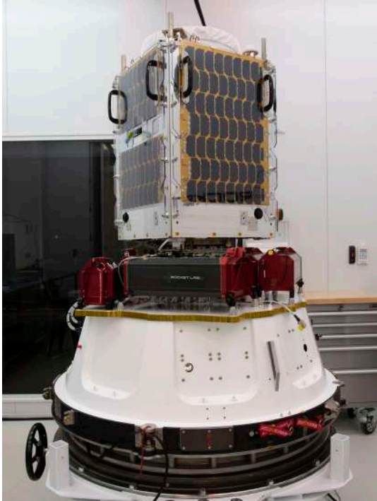
Figure 21 Flight 13 payload configuration
