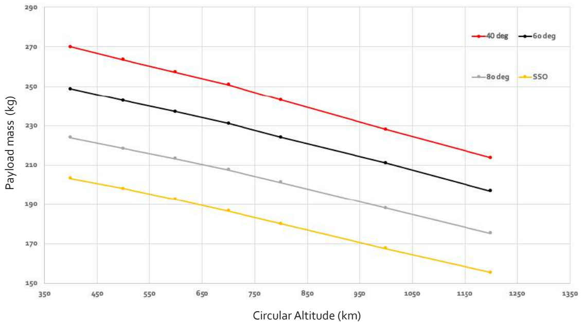
Figure 33 Performance to Circular Orbits
