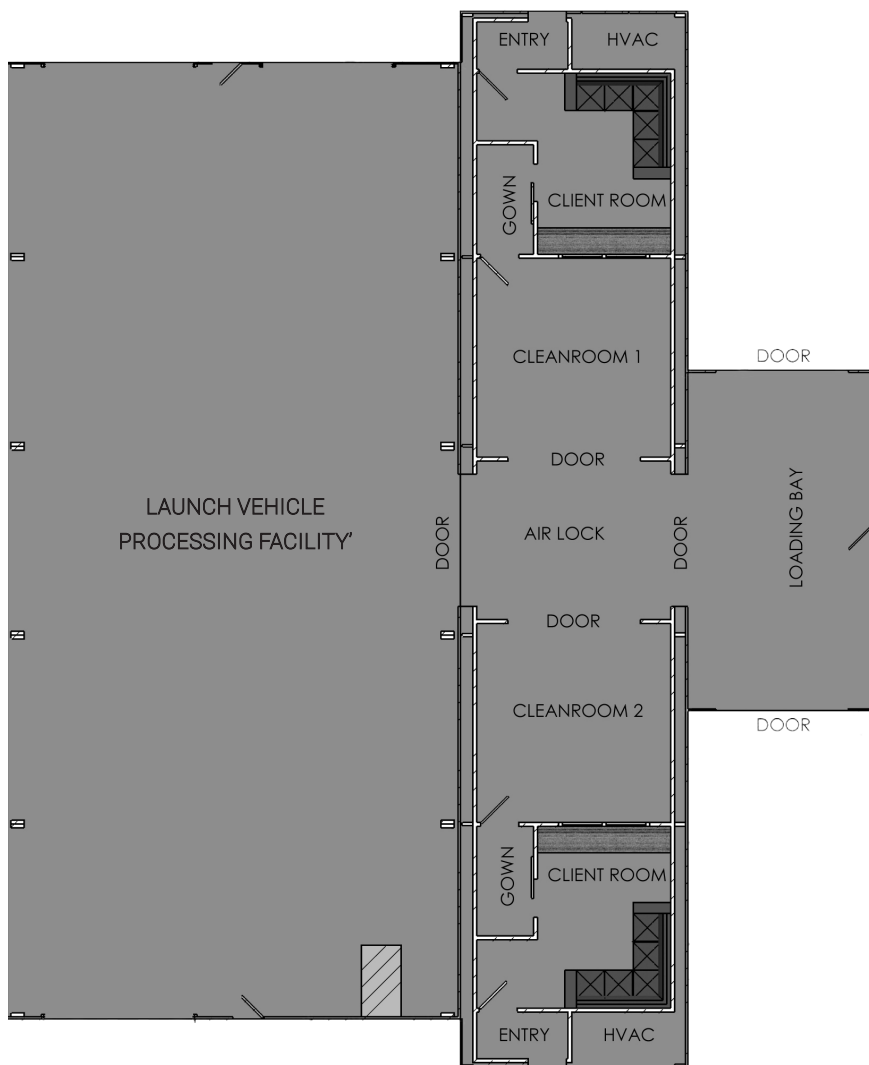
Figure 58 The layout of the Payload Processing Facility at LC-1
