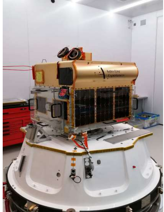
Figure 22 Flight 10 payload configuration
