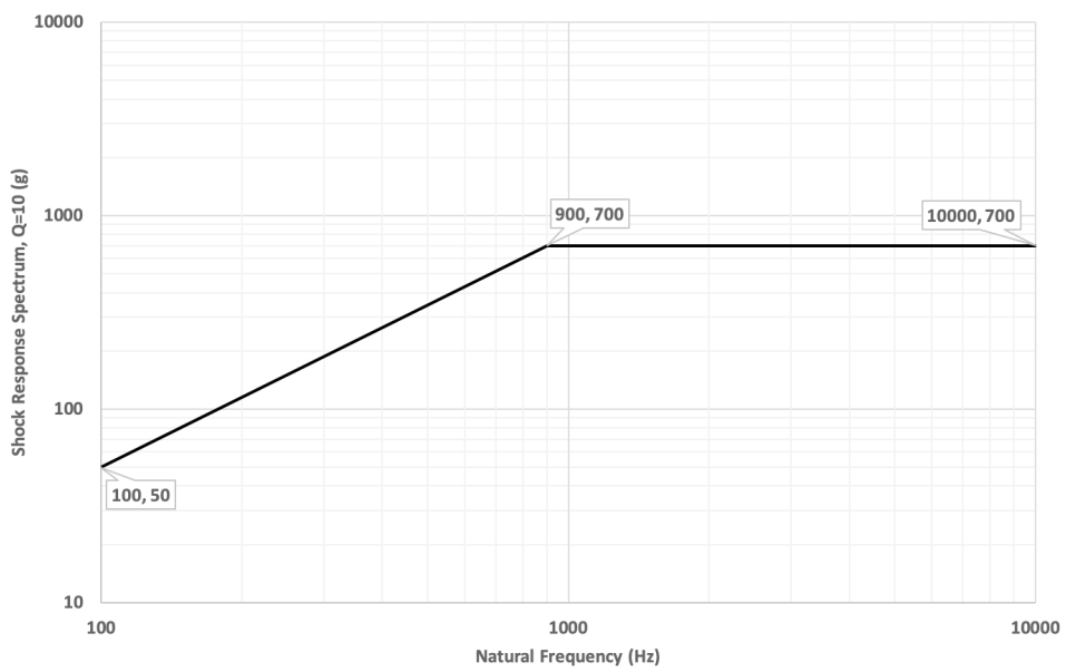
Figure 37 Electron Shock MPE
