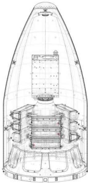
Figure 16 1 Microsat with 9 Cubesats
