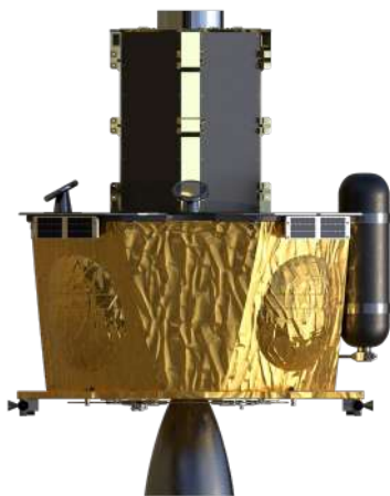
Figure 13 Photon Interplanetary Configuration
