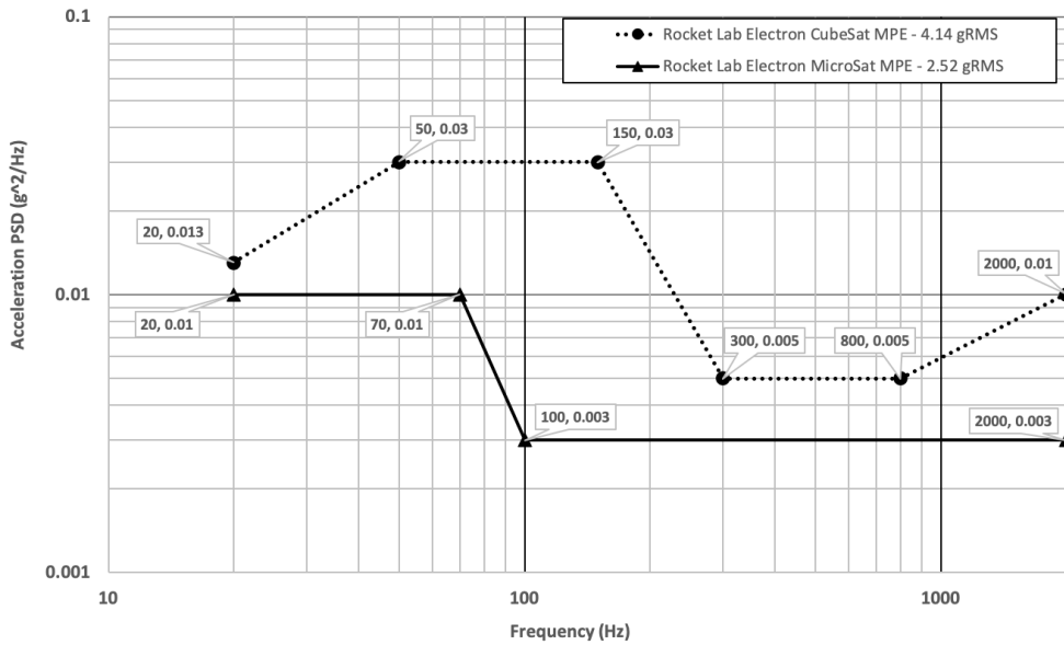
Figure 39 Electron Random Vibration MPE
