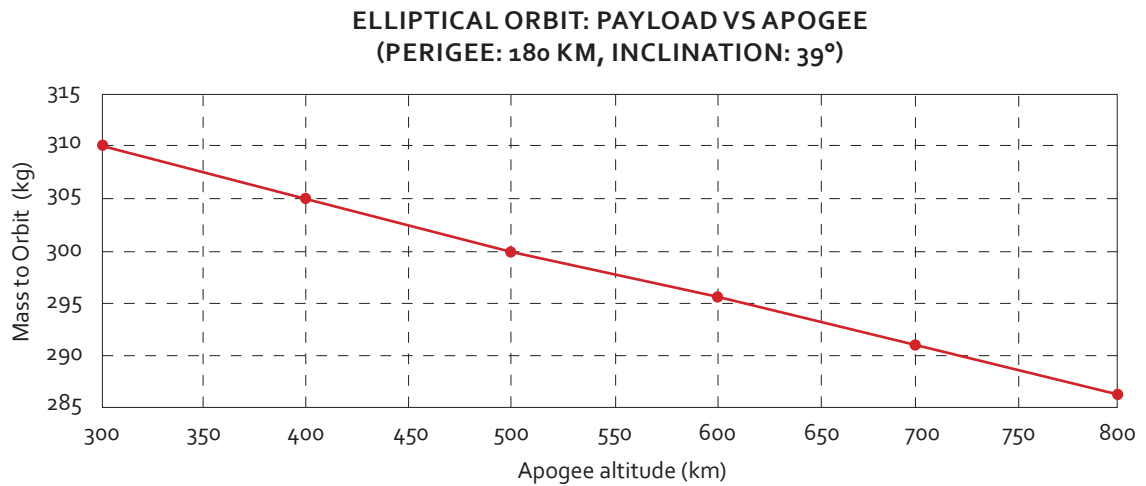
Figure 34 Performance to a 180 km Perigee at 39° Inclination Elliptical Orbit
