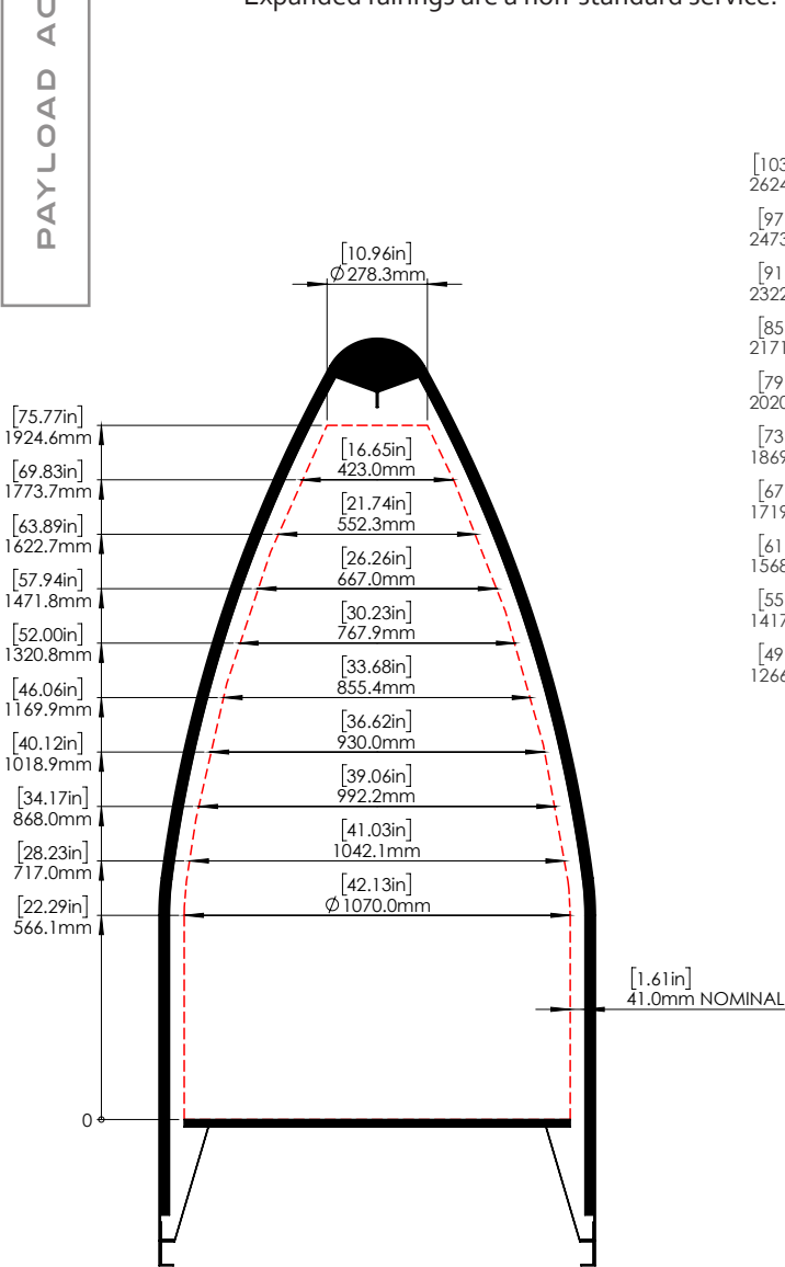
STANDARD ELECTRON FAIRING
