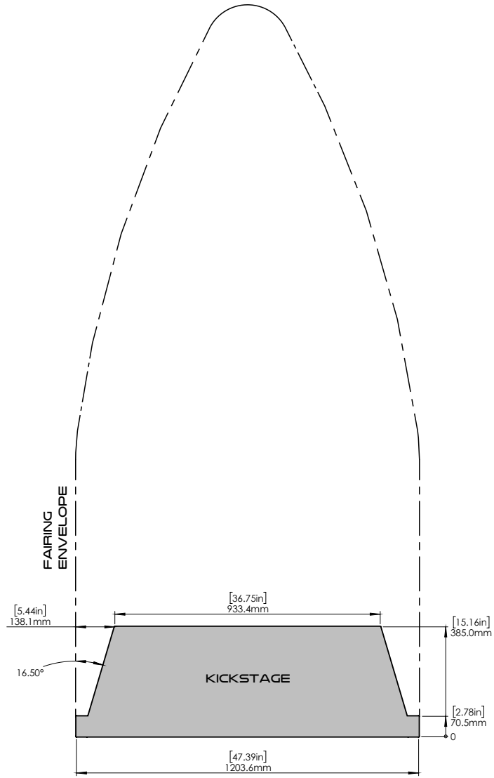
Figure 9 Electron fairing envelope
