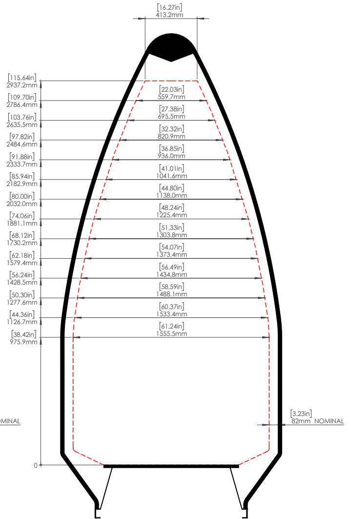
EXPANDED ELECTRON FAIRING
