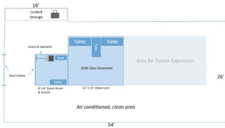
Figure 61 Rocket Lab's Long Beach Payload Processing Facility Layout
