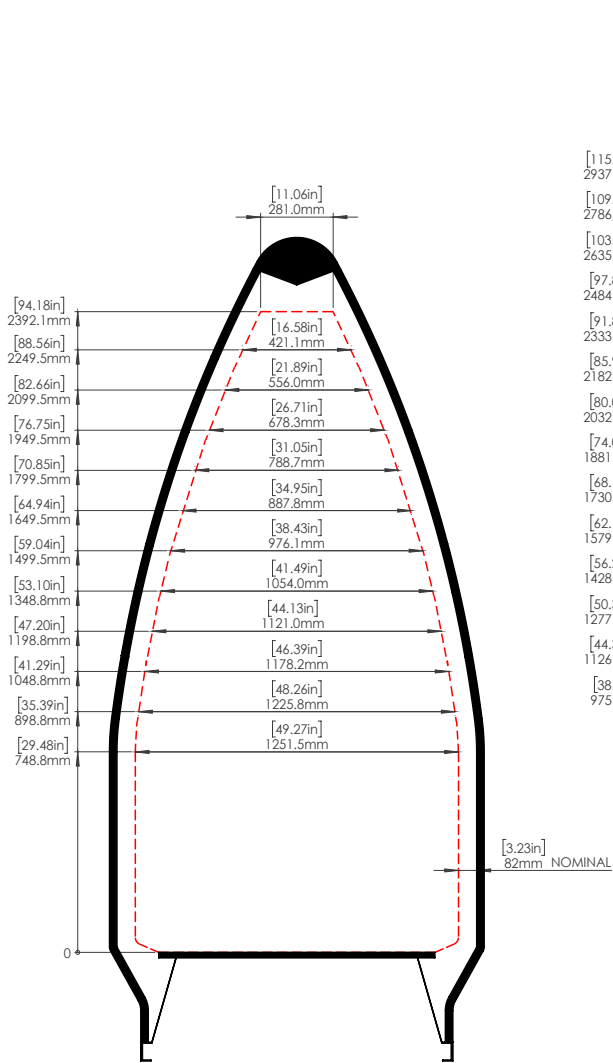
EXPANDED ELECTRON FAIRING (1.2X STANDARD)
