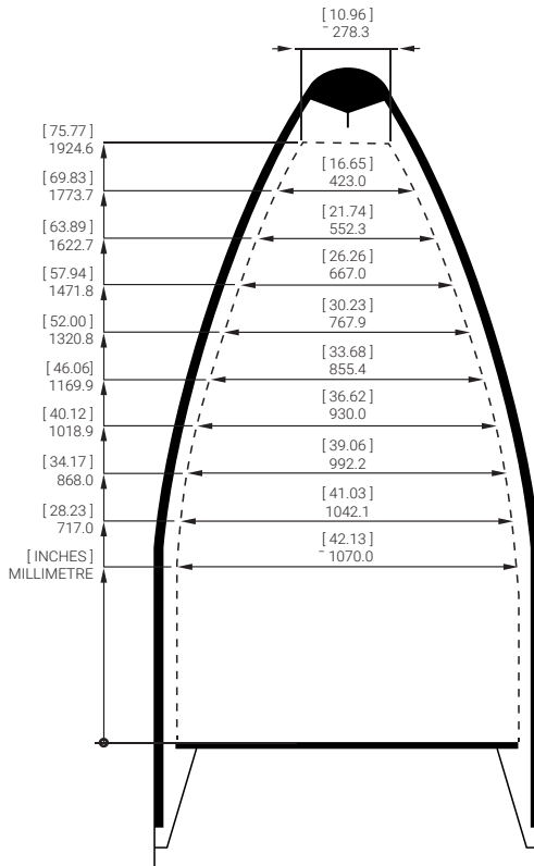
Figure 15 Fairing capacity & exterior of fairing
