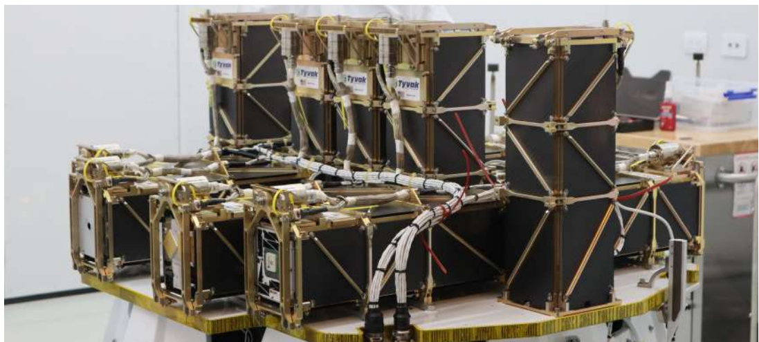
Figure 24 Flight 4 payload configuration
