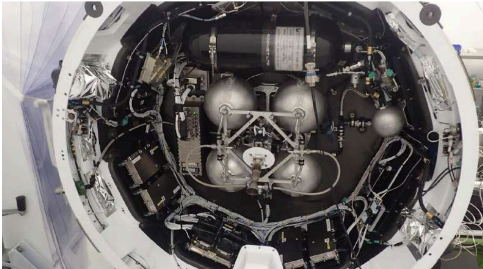
Figure 7 Rocket Lab's Kick Stage (aft View, Kickstage Interior)
