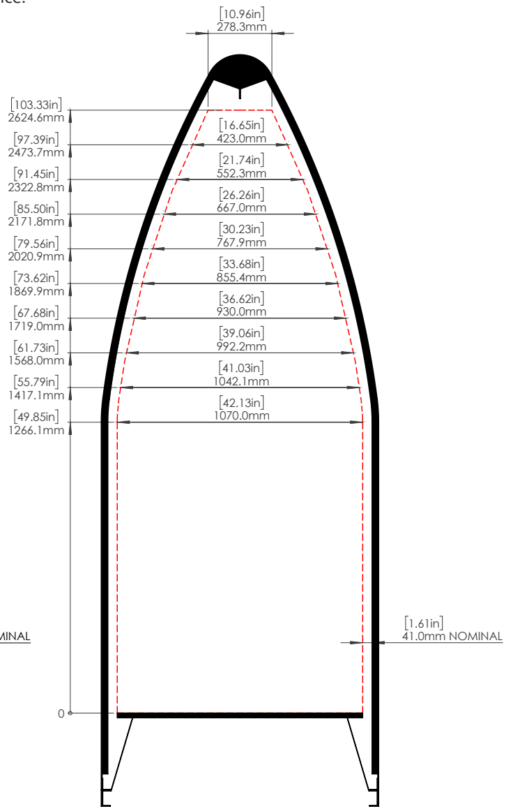
EXTENDED ELECTRON FAIRING
