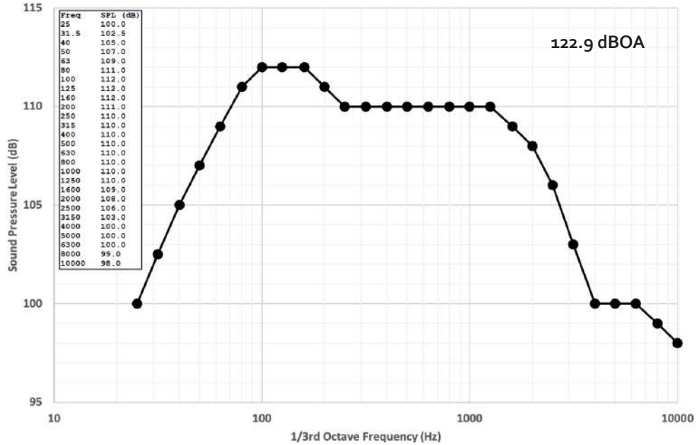
Figure 38 Electron Acoustic MPE
