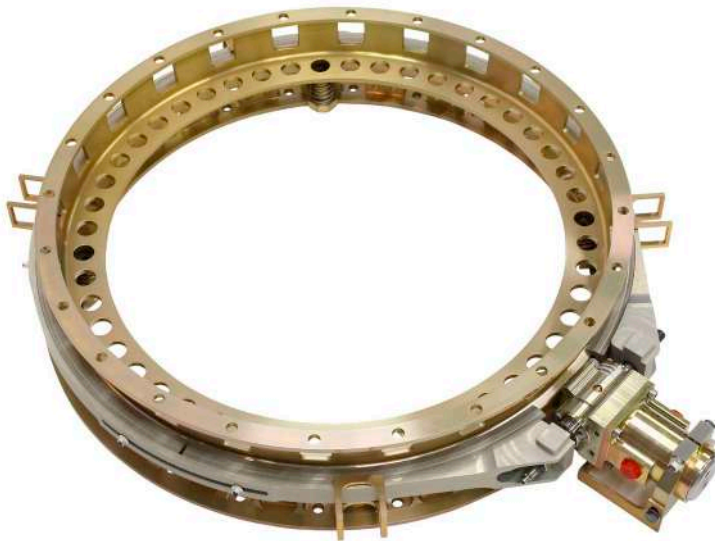
Figure 31 PAS 381S separation system
