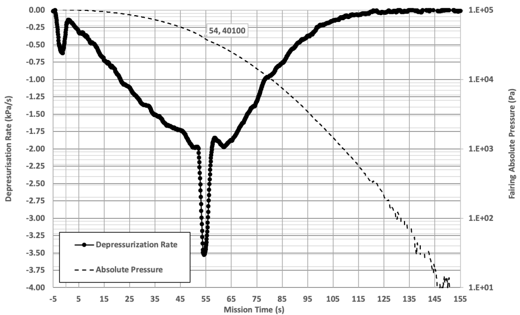
Figure 40 Electron Typical Fairing Venting Environment
