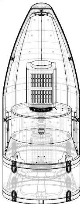
Figure 19 Dual stacked microsats on two Kick Stages
