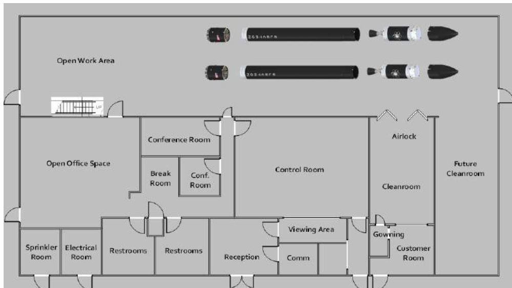
Figure 60 The layout of the Payload Processing Facility at LC-2
